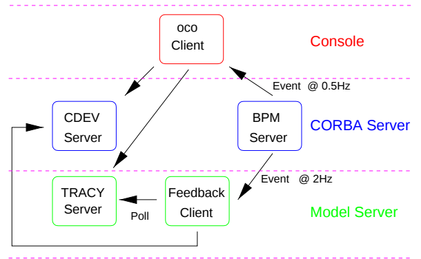
Figure 1: Schematic View of the SOFB: the “Feedback Client” on the “Model Server” level replaces the operator driven GUI “oco Client” on the “Console” level. The client gets BPM data from the “BPM Server”, asks the “TRACY Server” for the corresponding model predicted corrector settings and applies the correction through the “CDEV Server”
