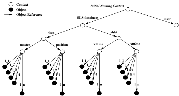
Figure 3: A naming graph for implementing database object references
