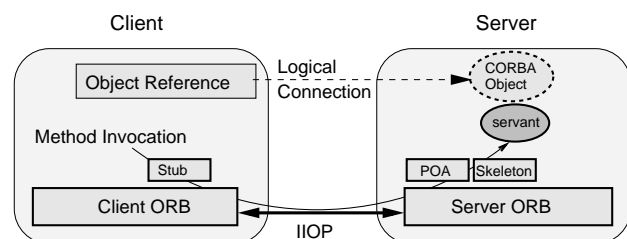
Figure 1: The CORBA client-server architecture
